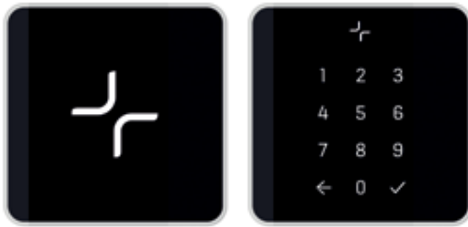
Figure 4: Card reader and card reader PIN unit (surface mounted), 88.5 x 88.5 x 20 mm
