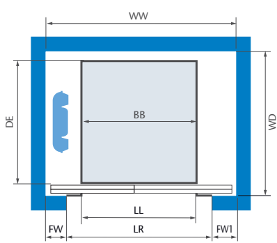
CAR WITHOUT FRONT WALL, DOOR LL = BB*
