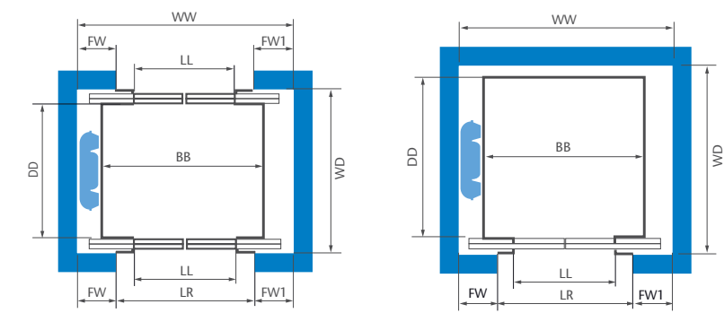
CAR WITH FRONT WALL, DOOR LL = BB*
